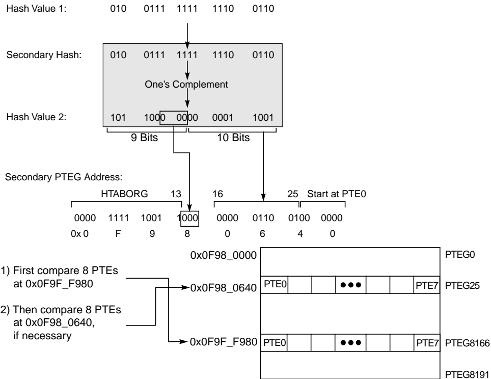
Figure 7-38. Example Secondary PTEG Address Generation—32-Bit Implementations
