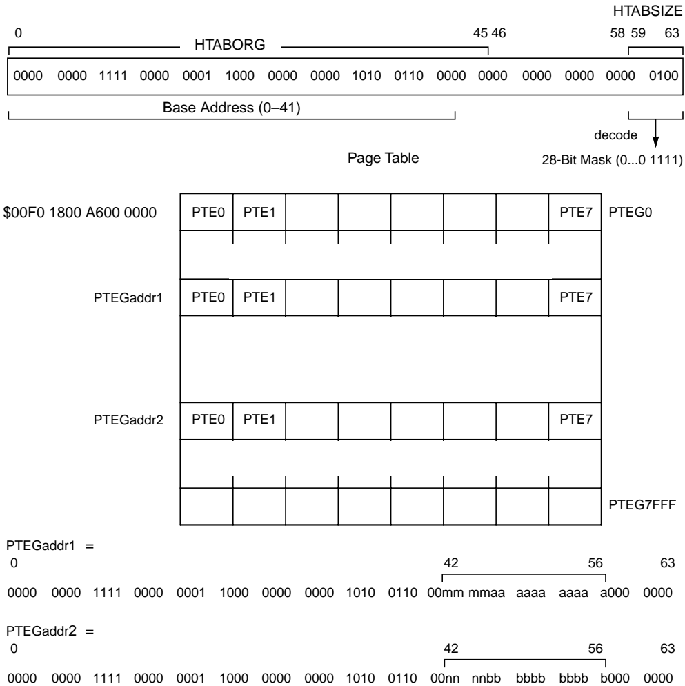
Figure 7-33. Example Page Table Structure—64-Bit Implementations
